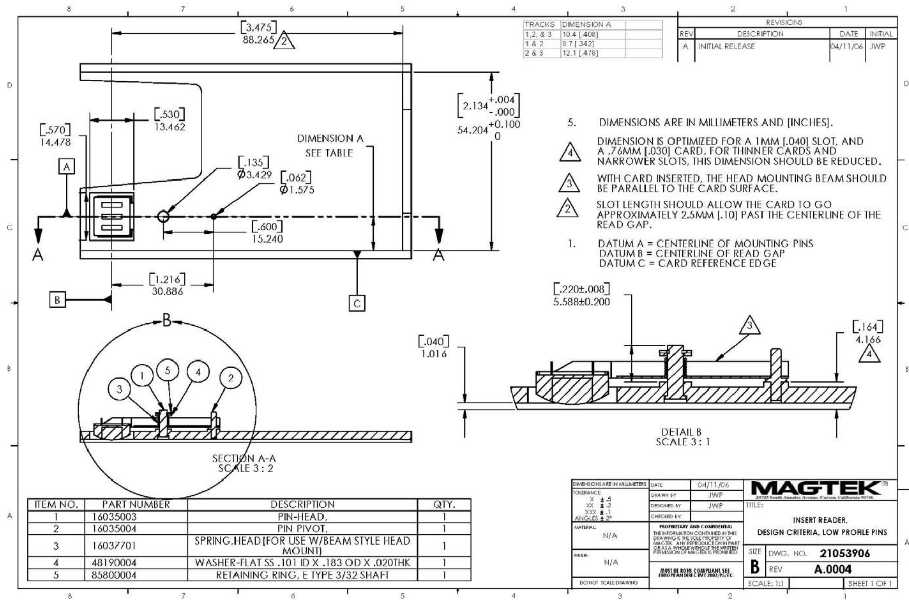
Figure A-11. Insert Reader Design Criteria
